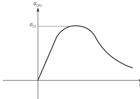
Figure 8 : Load-end shortening curve \sigma_{CR1}-\epsilon for beam column buckling
