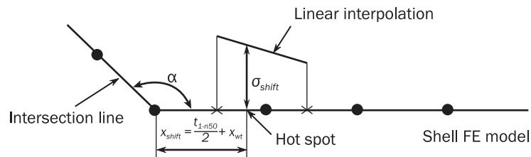
Figure 20 : Determination of stress read out points for web-stiffened cruciform connections
