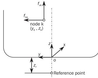
Figure 20 : Station forces and acting location of torsional moment at section
