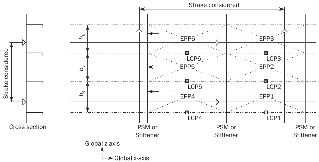
Figure 18 : Load calculation point (LCP) for longitudinal framing
