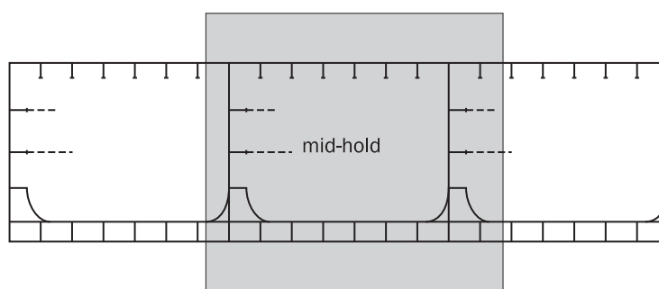
Figure 22 : Longitudinal extent of evaluation area for bulk carrier
