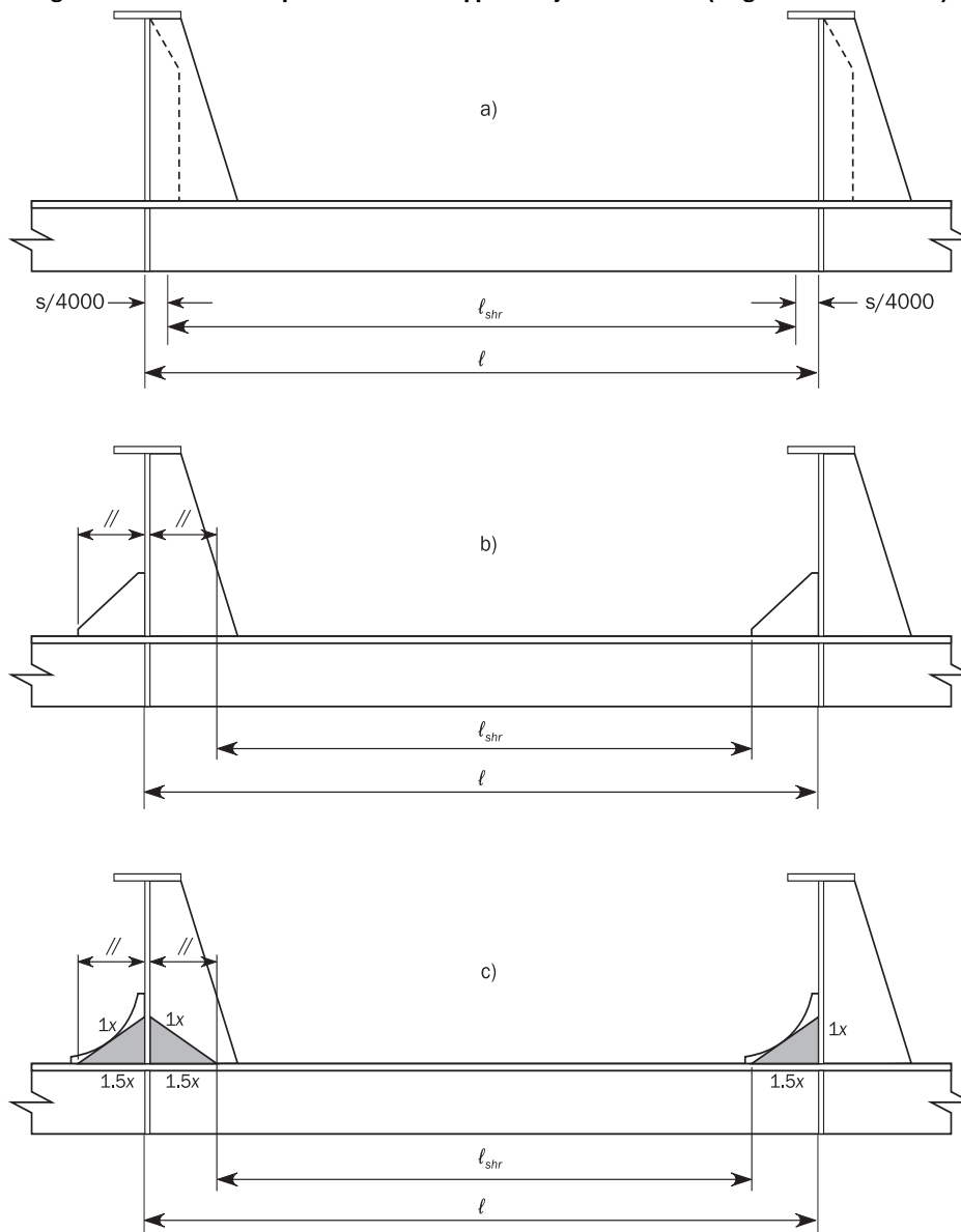
Figure 4 : Effective shear span of stiffeners supported by web stiffeners (single skin construction)
