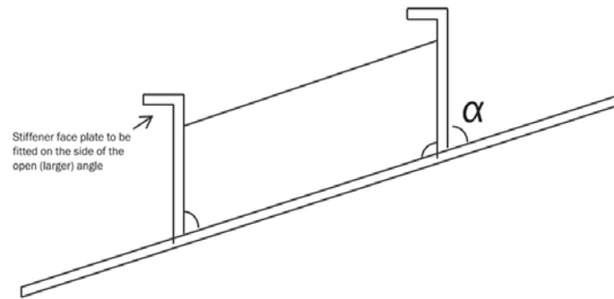
Figure 2 : Stiffener on attached plating with an angle less than 50 deg
