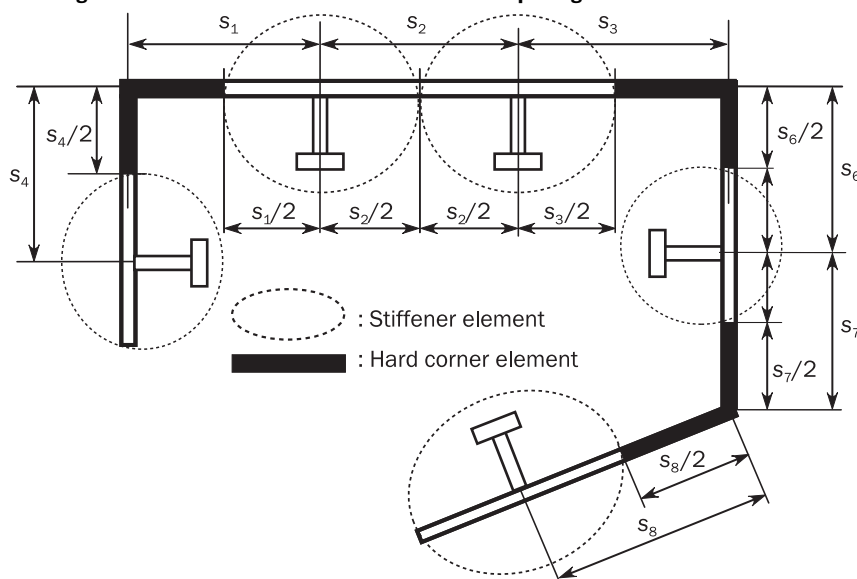
Figure 4 : Extension of the breadth of the attached plating and hard corner element
