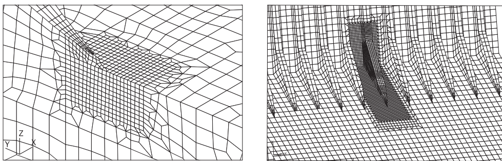
Figure 10 : Fine mesh zone around an opening
