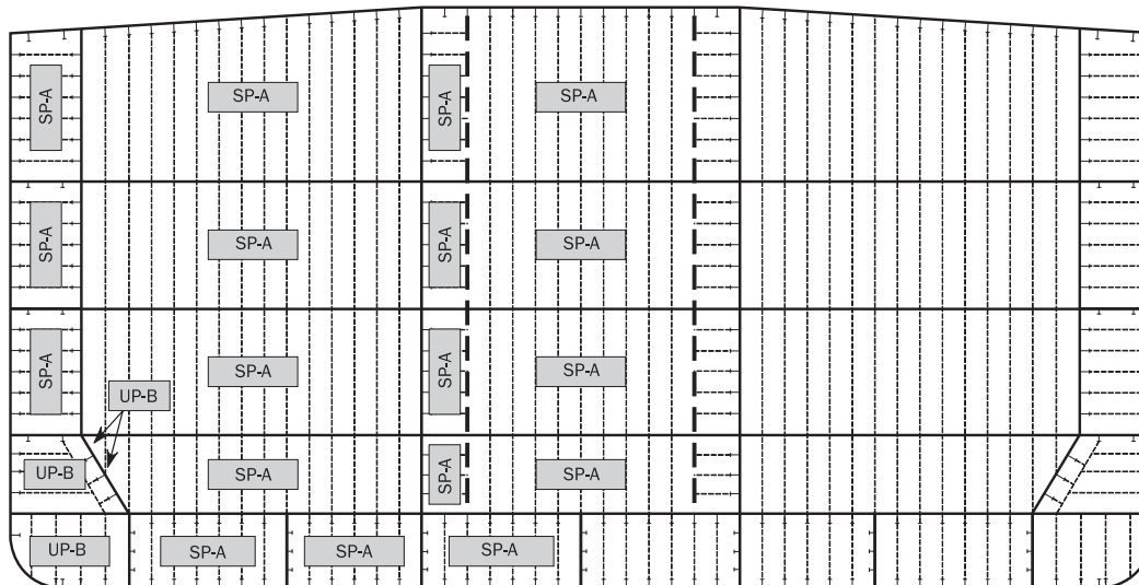
Figure 4 : Cross tie
