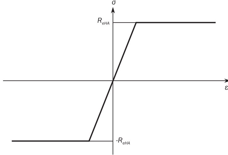
Figure 7 : Load-end curve \sigma - \varepsilon for elasto plastic collapse
