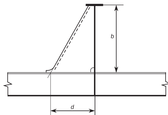
Tripping bracket in way of stiffener
