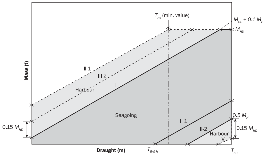
Example BC-A ships having {No MP} for FA hold
