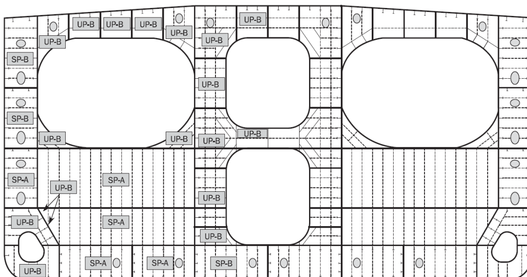
Figure 4 : Cross tie
