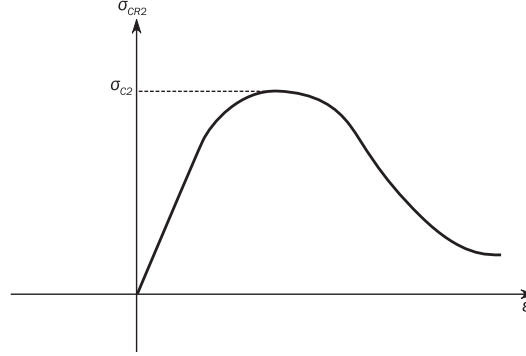
Figure 9 : Load-end shortening curve \sigma_{CR2} - \epsilon for flexural-torsional buckling
