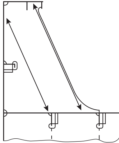
Figure 7 : Coaming stay (example 2)
