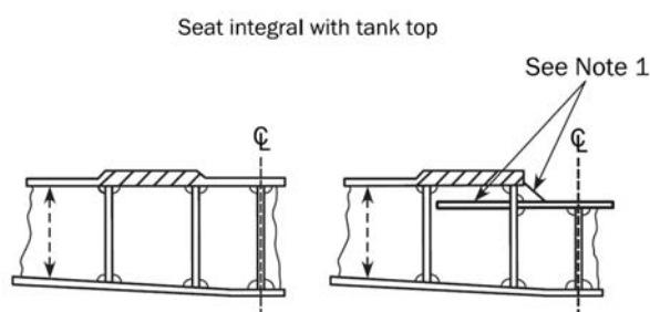
Figure 1 : Machinery foundations Type 1
