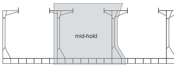
Figure 22 : Longitudinal extent of evaluation area for bulk carrier
