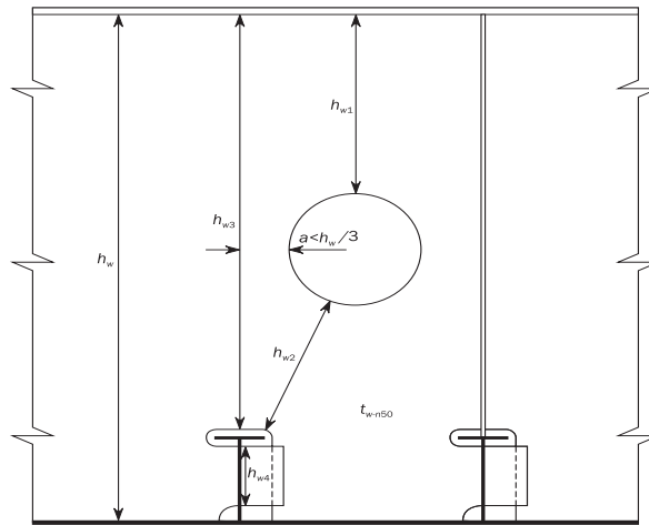
Figure 15 : Effective shear area in way of web openings
