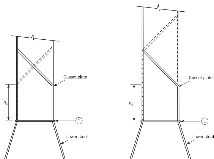
Figure 5 : Symmetrical and unsymmetrical gusset / shedder plates
