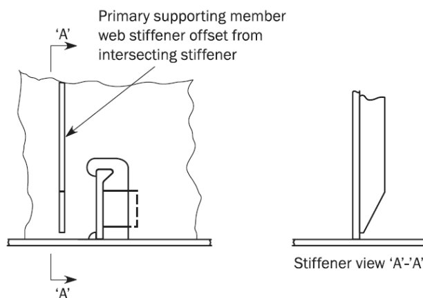
Figure 10 : Offset PSM web stiffeners
