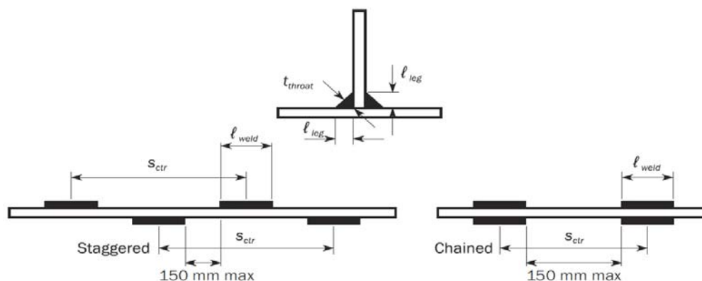
Figure 4 : Weld scantlings definitions
