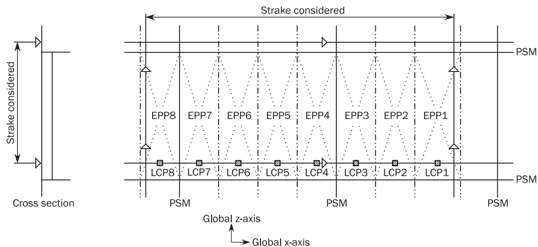
Figure 19 : Load calculation point for transverse framing
